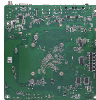
▲ Rear view
