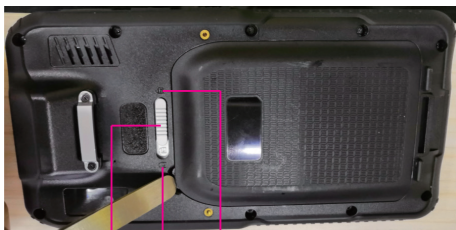
Battery latch Position of lock Position of unlock
